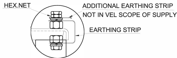
EARTHING ARRANGEMENT
