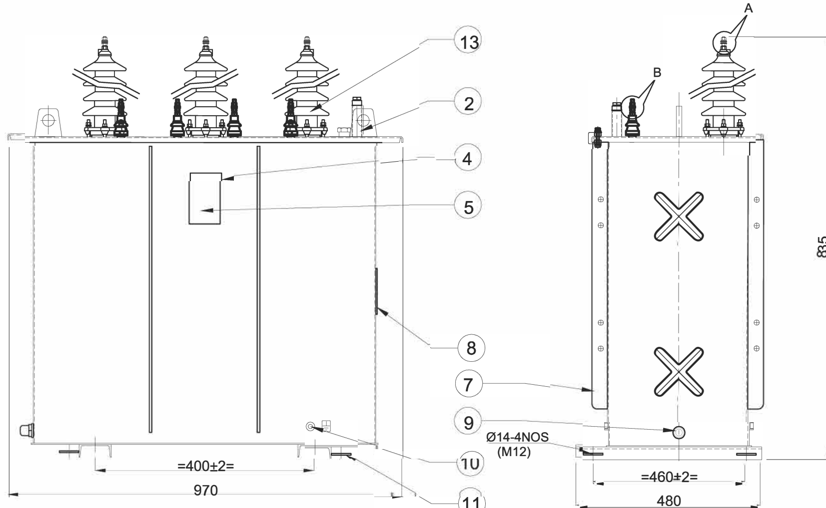
FRONT VIEW
